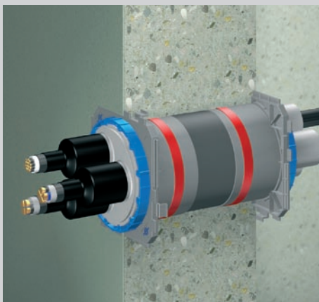
Curaline® BKD 150 Cable duct
